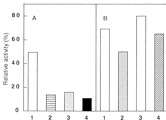
Figure 4. Inhibition by gangliosides of lectin – \kappa -casein interaction. (A) Wells were coated with \kappa -casein (20 \mu g), and lectin (0.5 \mu g) or lectin – ganglioside mixtures previously incubated in 10 \mu l PBS for 20 min were diluted five-fold with PBS and added to the wells. All the values were average of four determinations on the same plate. (1) D1a (1.4 nmol); (2) D1b (7 nmol); (3) M1a (7 nmol); (4) M1a (7 nmol) without lectin. The values were expressed as % relative to the absorbance ( A_{405} = 0.686 ) obtained with only lectin. (B) Differing from A, preincubation was not performed. All the values were average of three determinations on the same plate. 1, 20 \mu M NeuAc \alpha 2,3Gal \beta 1, 3GalNAc; 2, 40 \mu M NeuAc \alpha 2,3Gal \beta 1,3GalNAc; 3, 20 \mu M NeuAc \alpha 2,3Gal \beta 1,3(NeuAc \alpha 2,6)GalNAc; 4, 40 \mu M NeuAc \alpha 2,3Gal \beta 1,3(NeuAc \alpha 2,6)GalNAc. The values were expressed as % relative to the absorbance ( A_{405} = 0.808 ) obtained with only lectin.
