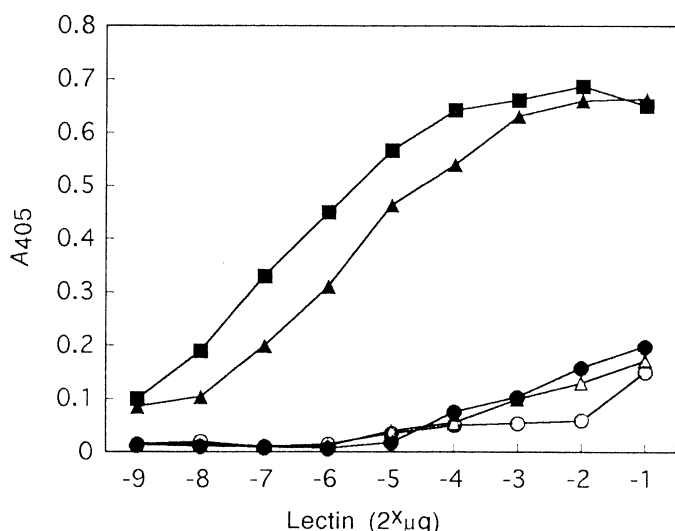
Figure 3. Binding of Agrocybe lectin to BSA-conjugates on ELISA plate. All the values were average of three determinations. Open circle, control (only BSA); closed circle, NeuAc \alpha 2,3Gal-BSA; NeuAc \alpha 2,3Gal \beta 1,3GlcNAc-BSA, ■; and NeuAc \alpha 2,3Gal \beta 1,4GlcNAc-BSA, ▲; murine laminin, \Delta .
