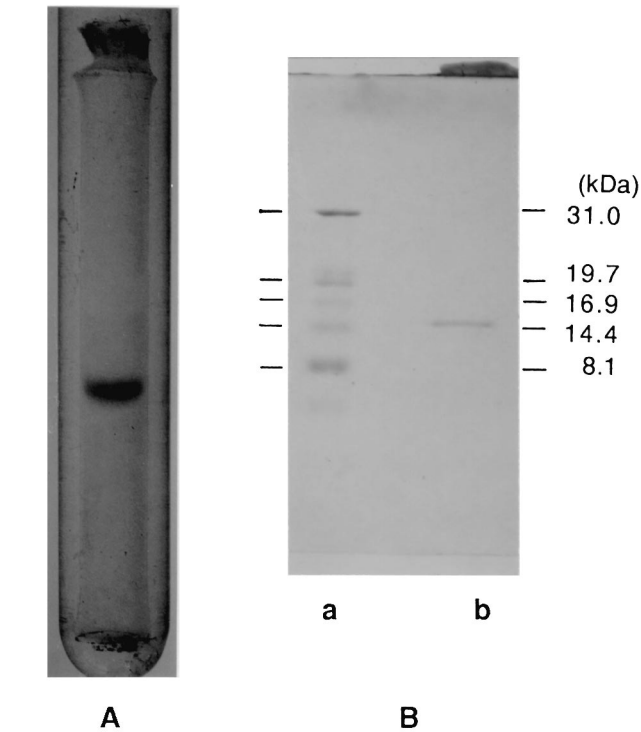
Figure 2. Results of PAGE and SDS-PAGE of the final preparation. (A) PAGE (7.5% gel) at pH 8.9; (B) SDS-PAGE (15% gel), a and b, molecular-mass marker (Wako Pure Chemical, Osaka, Japan) and Agrocybe lectin in the absence of 2-mercaptoethanol, respectively.
